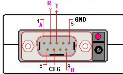
RS-232/485/422
